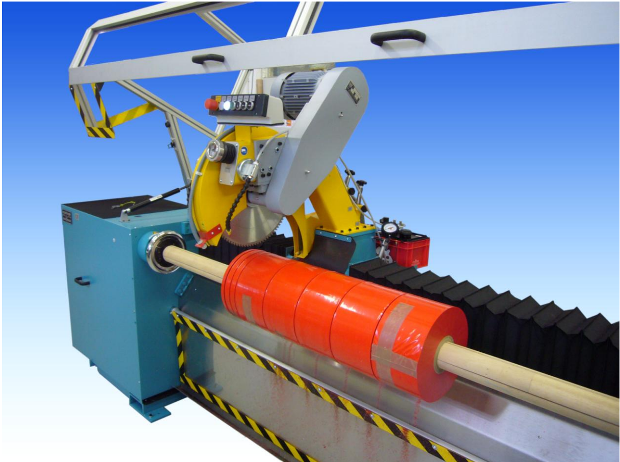
MOLEY® 500/1600 with Circular Saw Unit KRS
